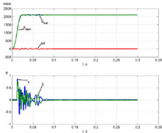
Fig. 3. Transient process signals with V_{max}=1m/s , a_{max}=15 m/s^2
